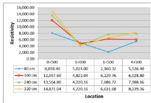
Fig. 5. Graph of Land Resistivity Measurement
