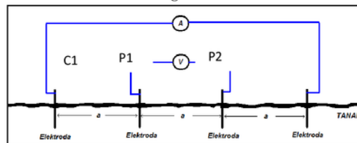
Fig. 2. Measurement of soil resistance with four Wenner electrode (Source: Adi. 2008).
