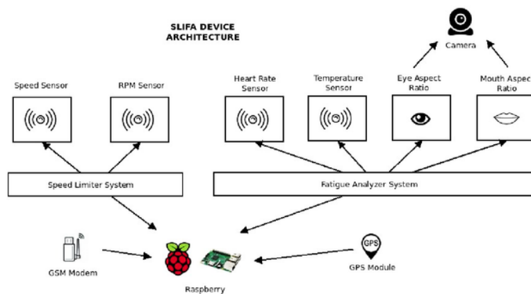
Figure 7. Architecture of SLIFA device
