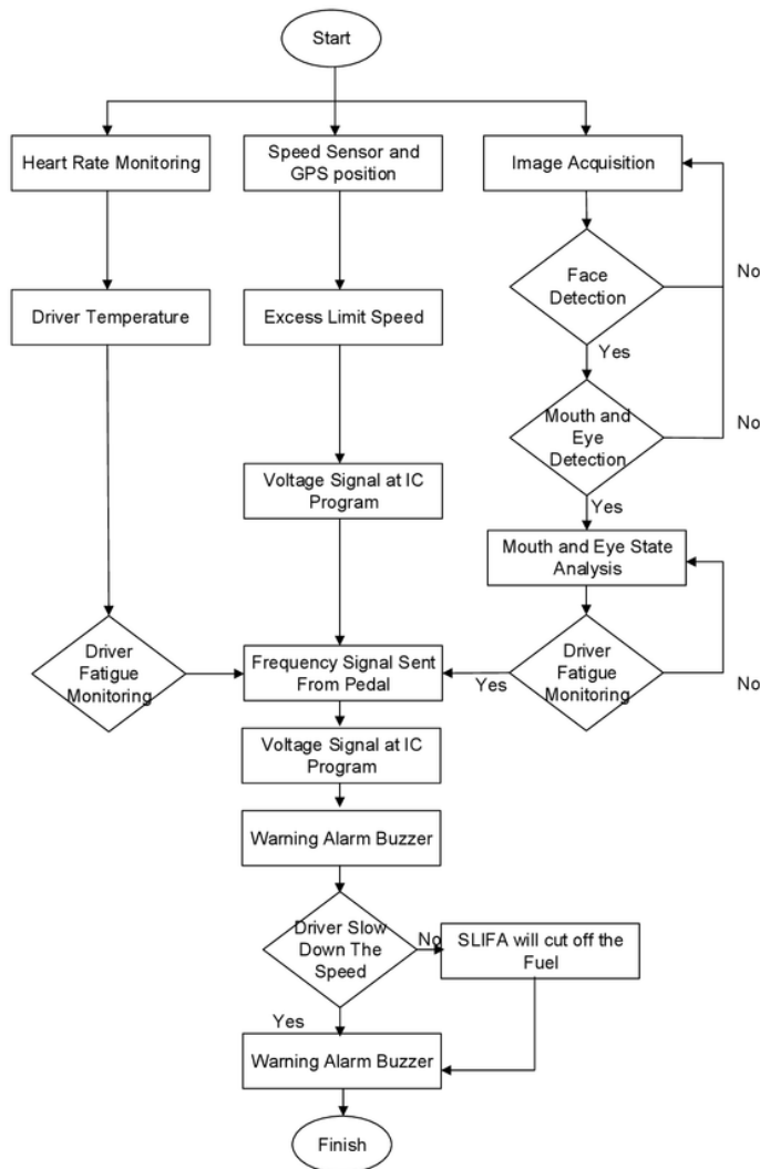
Figure 3. Limiter speed schematic
