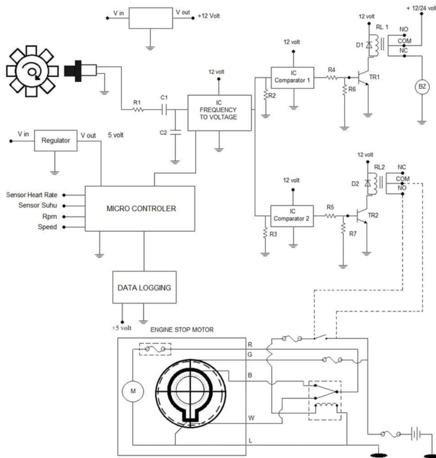
Figure 14. Completed block circuit of the SLIFA
