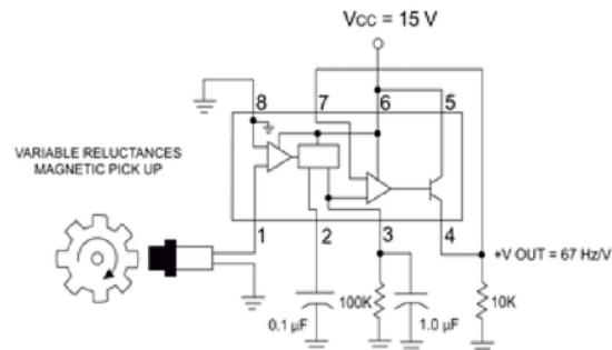
Figure 6. Minimum component tachometer diagram
