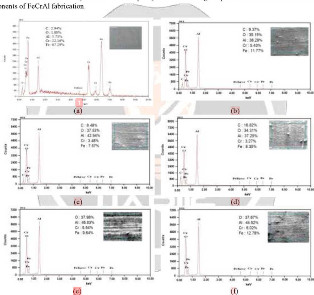
Fig -3: Composition analysis of (a) Raw material; (b) UB 1 hour; (c) UB 1.5 hour; (d) UB 2 hour; (e) UB 2.5 hour and (f) UB 3 hour
