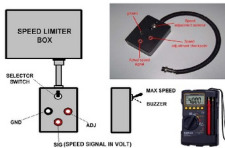
Fig. 4 Speed Calibration Test
