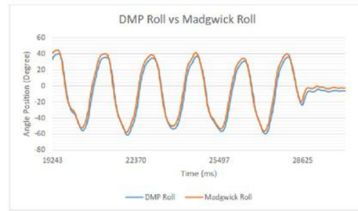
Figure 17: Angular position: DMP roll vs. Madgwick roll
