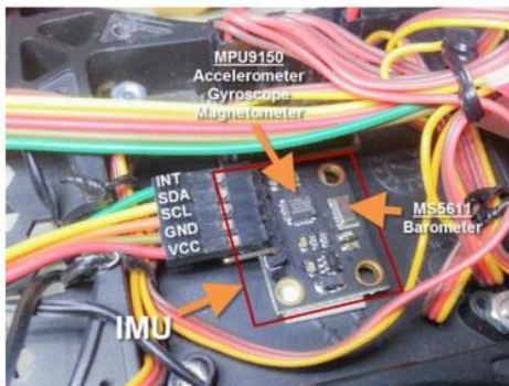
Figure 9: IMU unit and DMP
