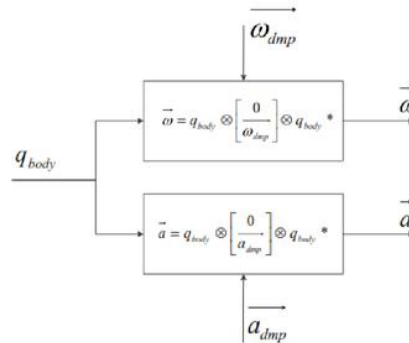
Figure 7: Rotational speed and acceleration calculation
