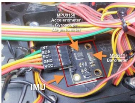
Figure 8: A UAV quadrotor system
