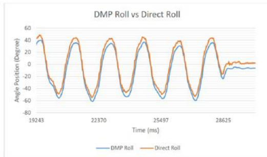
Figure 14: Angular position: DMP roll vs. direct AHRS roll
