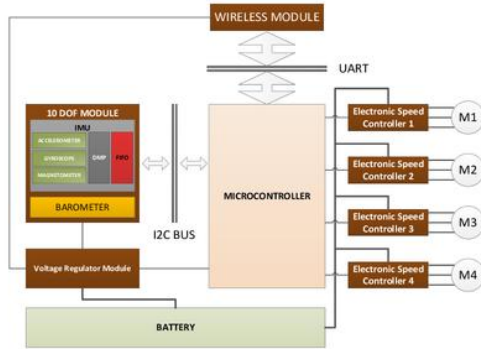
Figure 5: Block diagram of quadrotor system
