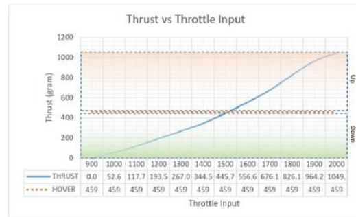
Figure 11: A UAV quadrotor maneuver test
