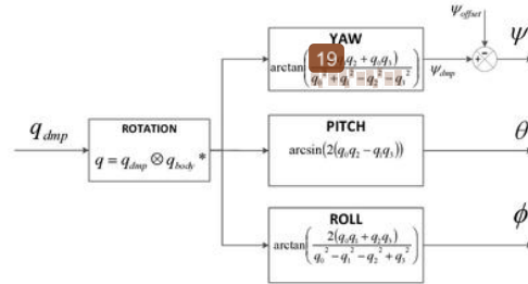
Figure 6: Angular position calculation
