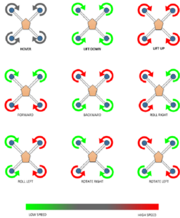
Figure 2: Coordinates and movement principle of quadrotor
