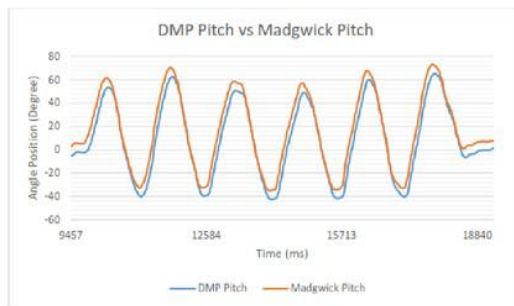
Figure 15: Angular position: DMP roll vs. Madgwick pitch
