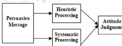
Figure 1: Heuristic-Systematic Model
