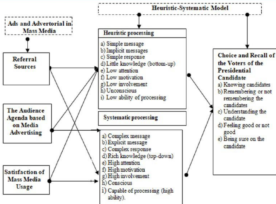
Figure 2: Framework
